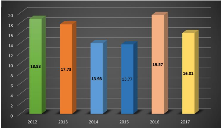
Gambar : 1 Rata-rata Hari Hujan (Hari), 2012-2017 Figures Average Rainy Days, 2012-2017
